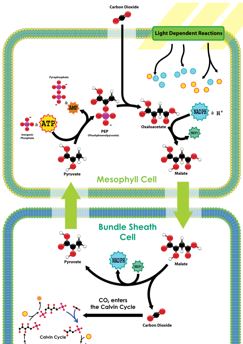
Overview of C4 carbon fixation
