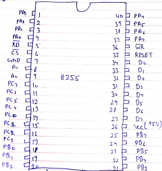
fig 1.1 Pin Diagram of 8255
