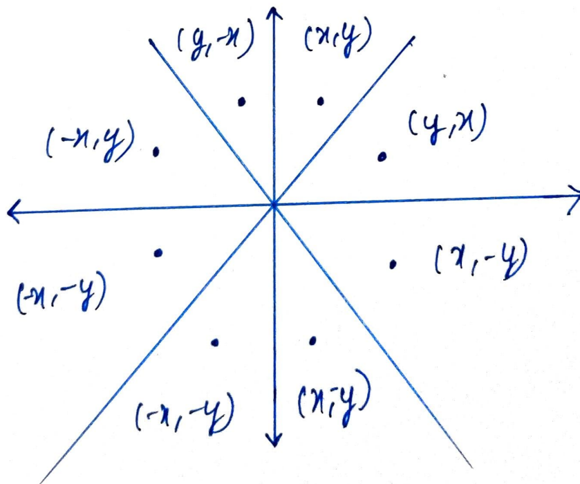
Fig: Eight way symmetry of circle.
