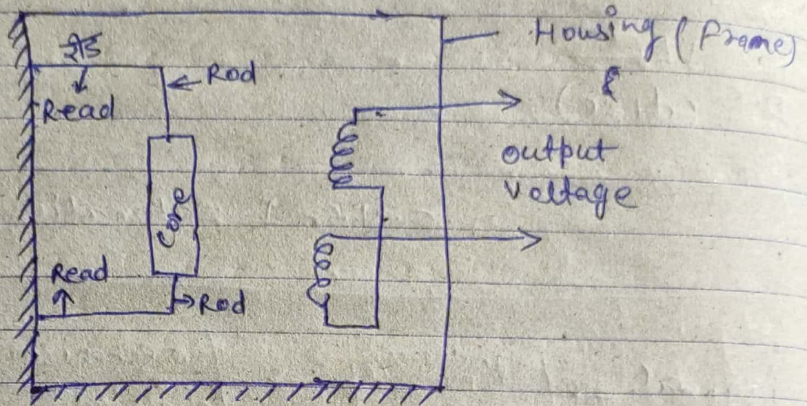
LVDT Accelerometer
