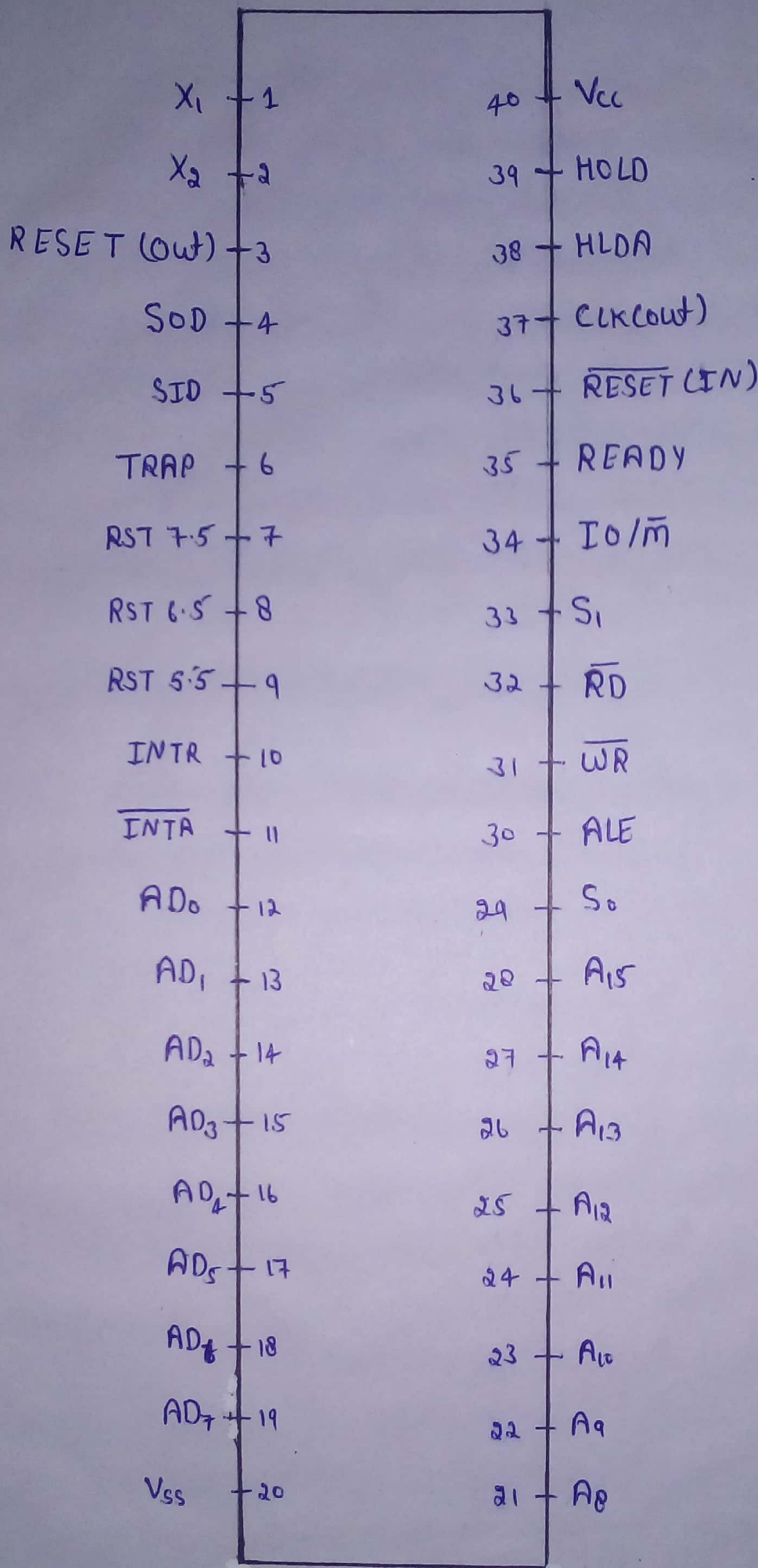
8085 - PIN DIAGRAM
