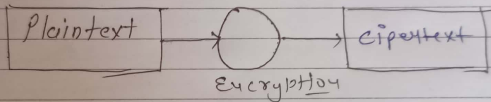
fig:-&gt; Encryption.
