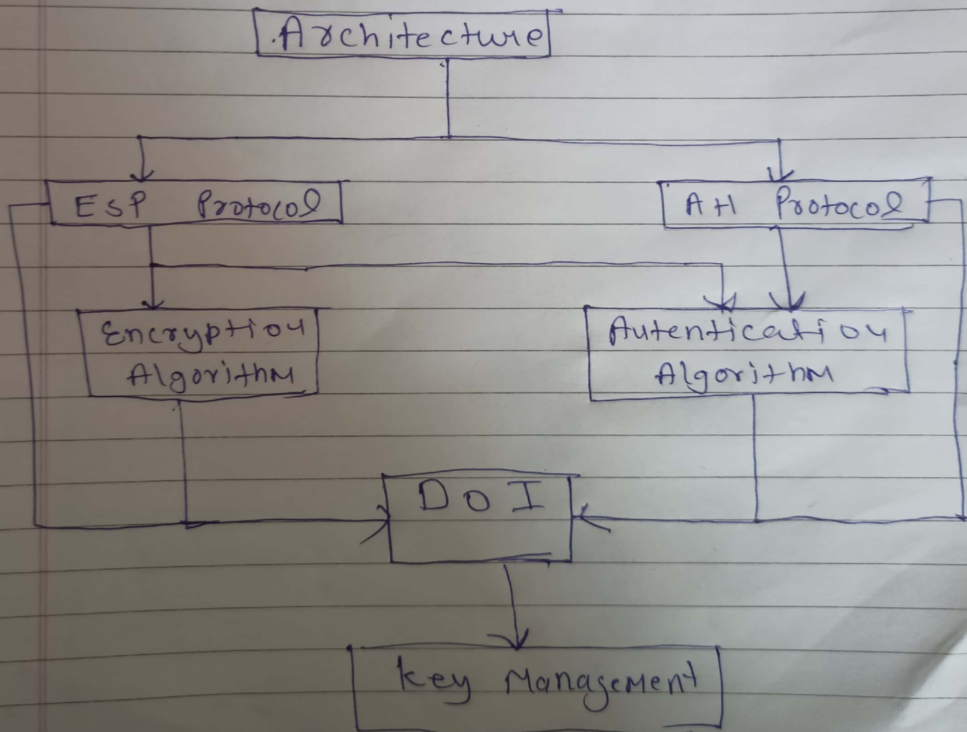
Fig:-> IP Security Architecture
