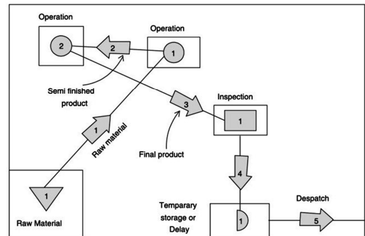
Figure 4.3 Flow Diagram
