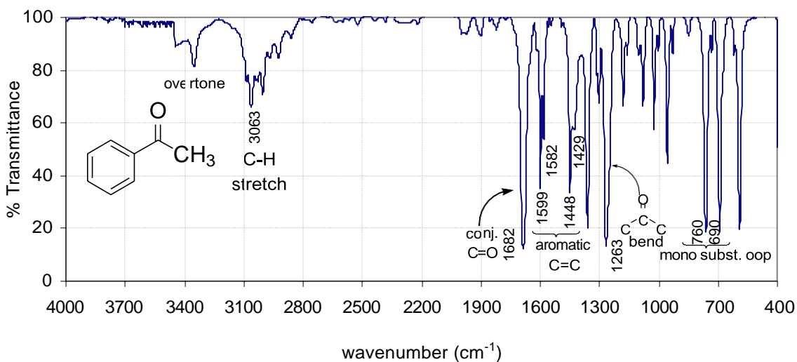
Figure 31 : The infrared spectrum of acetophenone (neat liquid)
