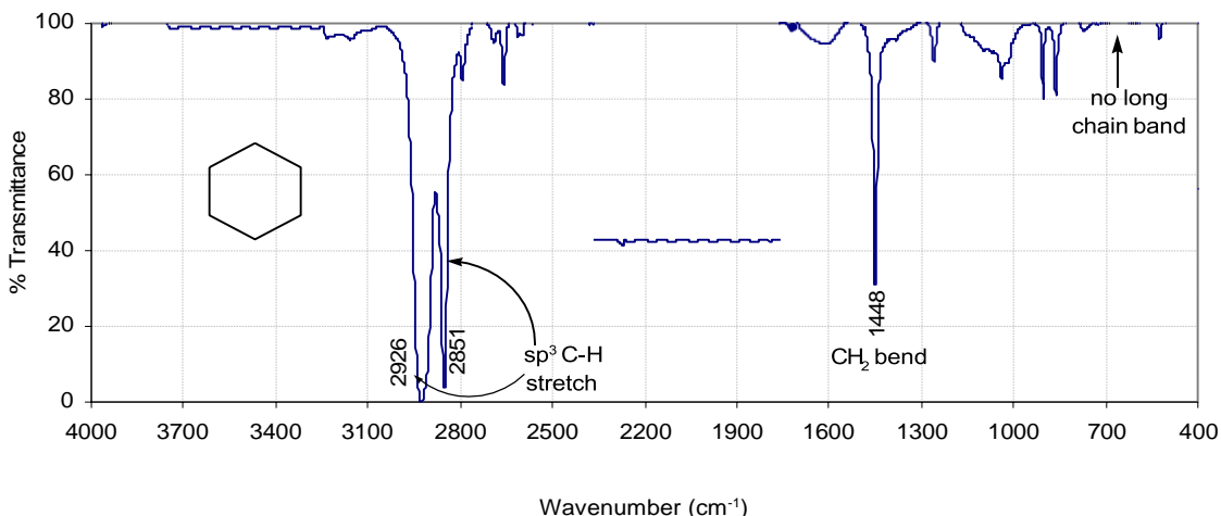
Figure 15 : The infrared spectrum of cyclohexane (neat liquid)
