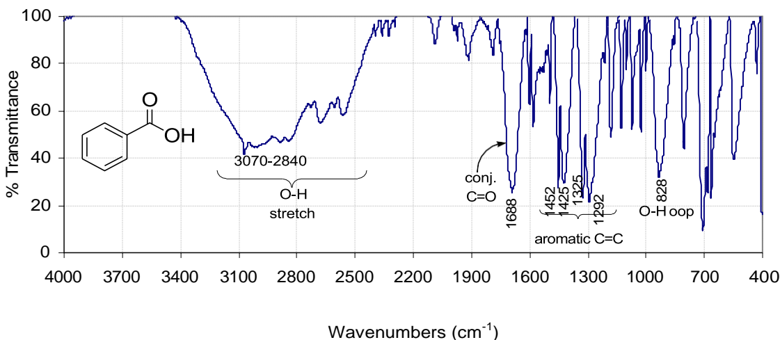
Figure 33 : The infrared spectrum of benzoic acid (nujol mull)
