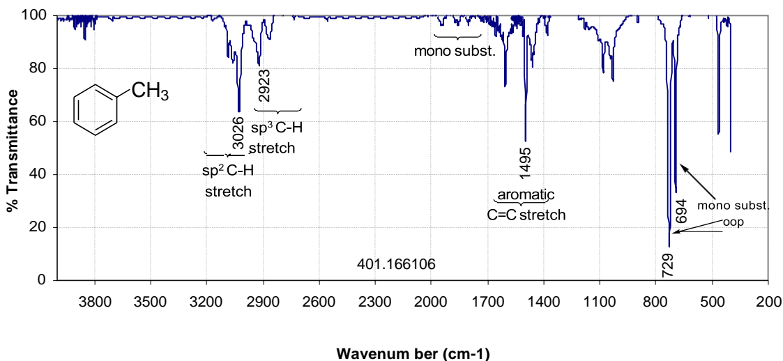
Figure 18 : The infrared spectrum of toluene (neat liquid)
