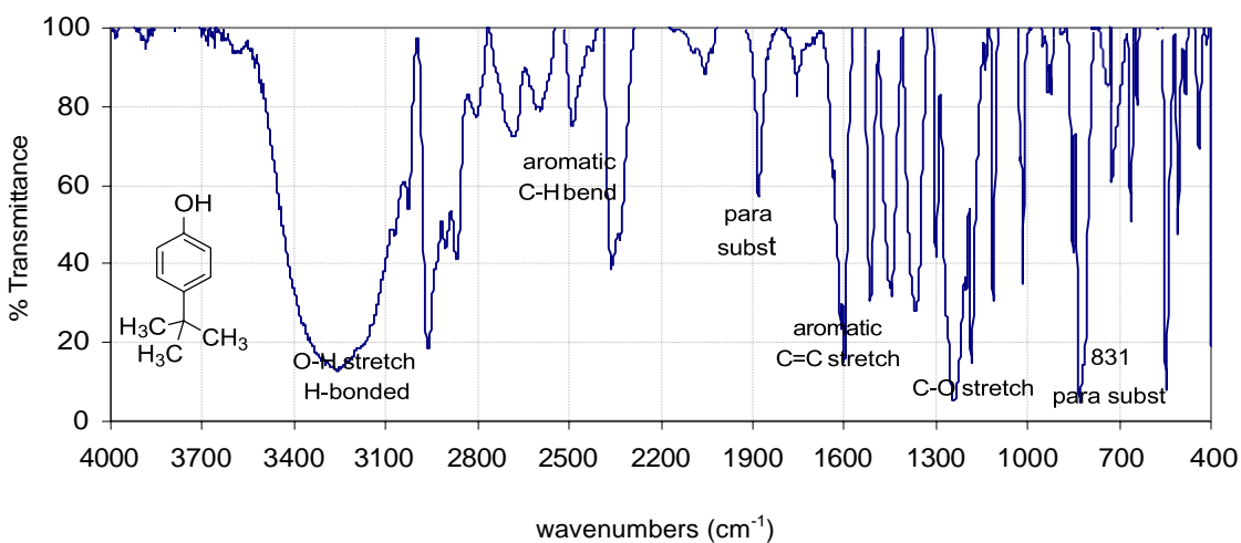
Figure 22 : The infrared spectrum of t -butylphenol (nujol mull)
