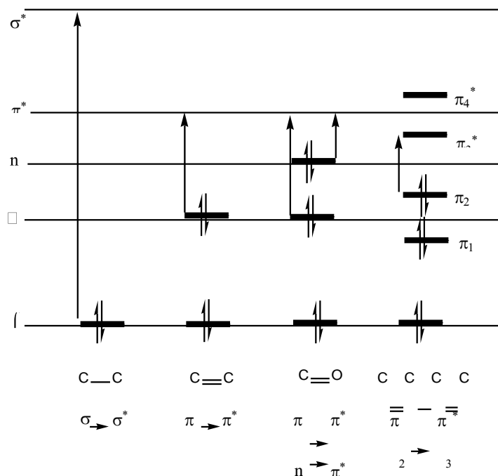
Figure 3 : Relative energies of orbitals most commonly involved in electronic spectroscopy of organic molecules
