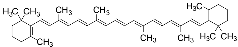
Figure 7: Structure of \beta -carotene
