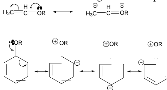
Figure 24 : The resonance effects in vinyl ethers and aryl alkyl ether
