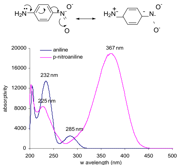
Figure 11 : UV-spectra of aniline and p -nitroaniline in methanol
