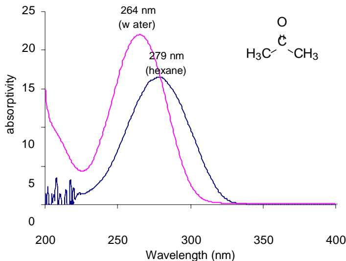
Figure 5 : UV-spectra of acetone in hexane and in water
