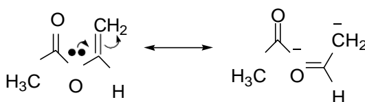
Figure 35 : Resonance effects in vinyl esters
