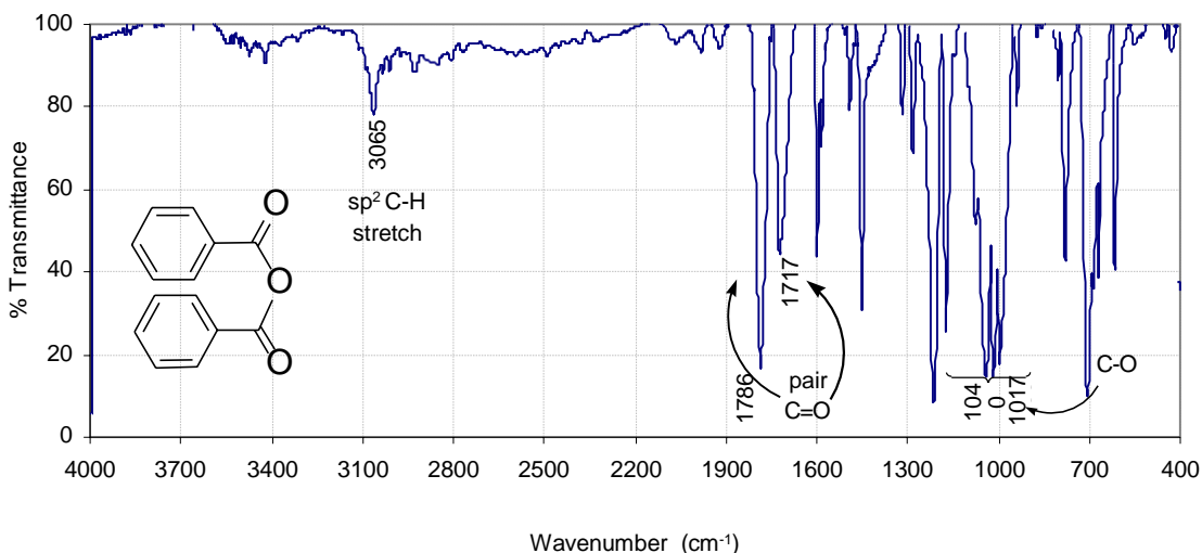
Figure 37 : The infrared spectrum of benzoyl anhydride (nujol mull)
