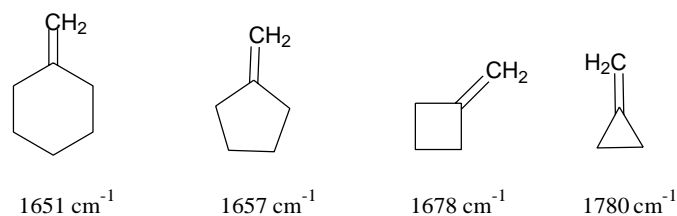
Figure 17 : Exocyclic C=C double bond frequencies in various ring sizes
