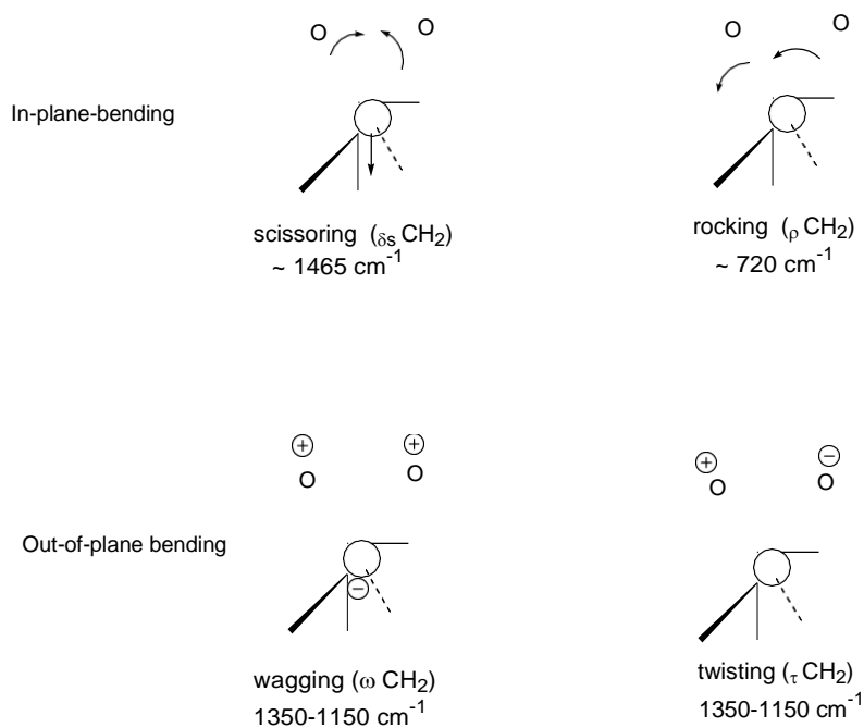
Figure 14: Vibrational modes of a CH 2 group. [ + and - indicate movement above and below the plane of page]
