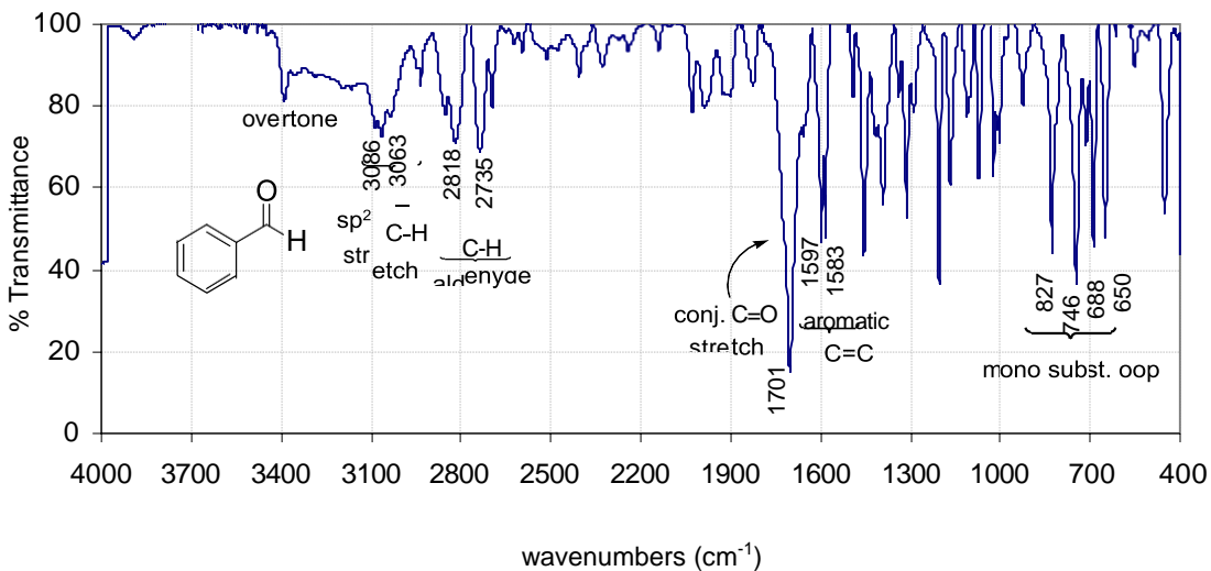
Figure 30 : The infrared spectrum of benzaldehyde (neat liquid)
