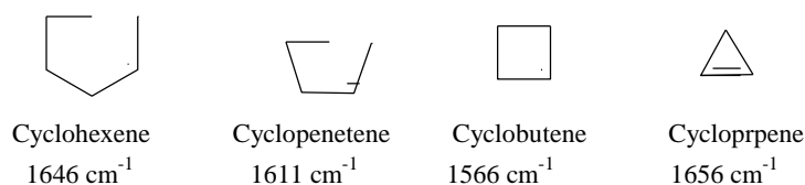
Figure 16 : C=C vibration frequencies of cycloalkenes
