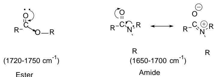
Figure 25 : Inductive and resonance effects in ester and amide groups
