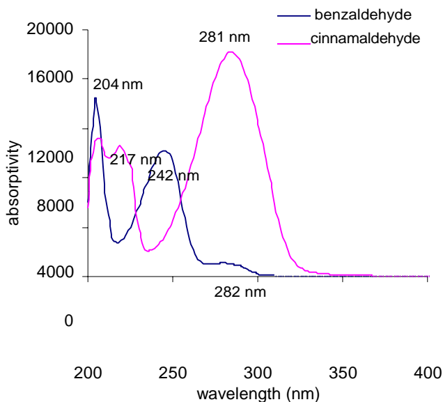
Figure 10 : UV-spectra of benzaldehyde and cinnamaldehyde in methanol
