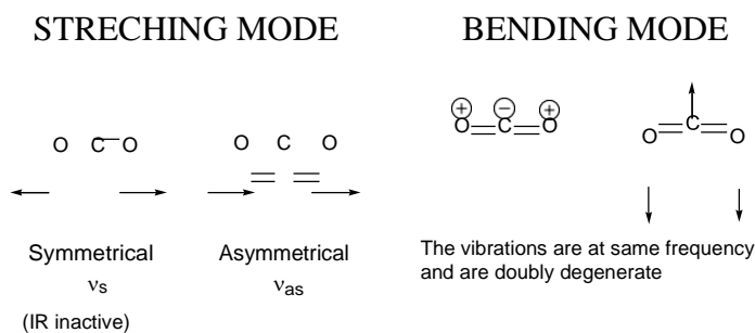
Figure 13: Vibrational modes for carbon dioxide molecule
