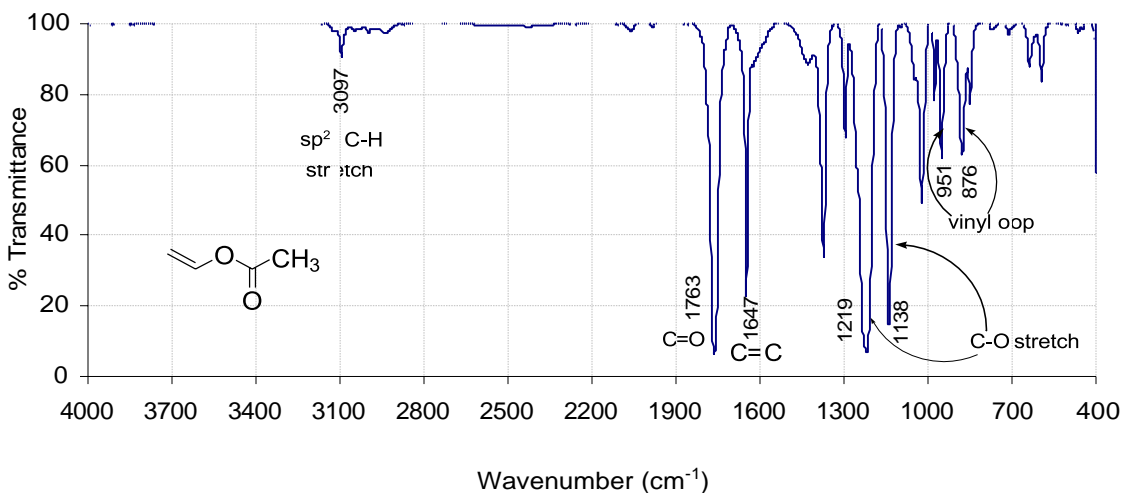
Figure 36 : The infrared spectrum of vinyl acetate (neat liquid)
