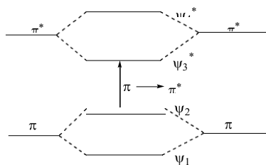
Figure 6 : Effect of conjugation on orbitals' energy and respective \pi - \pi^* transition.
