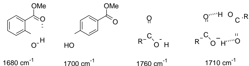
Figure 29 : H-bonding effects on C=O stretch
