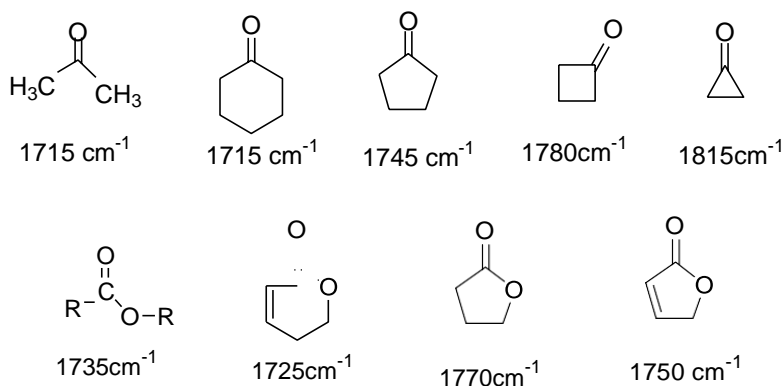
Figure 28 : C=O stretching frequencies in various compounds
