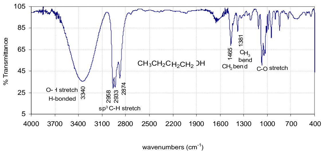
Figure 21 : The infrared spectrum of 1-butanol (neat liquid)
