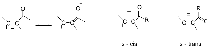
Figure 27 : Resonance effects and s-cis and s-trans structures in enones
