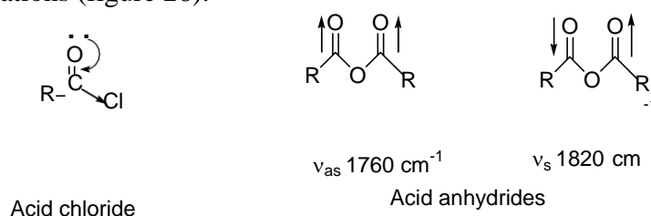
Figure 26 : Inductive effect in acid chloride and C=O stretch in anhydride
