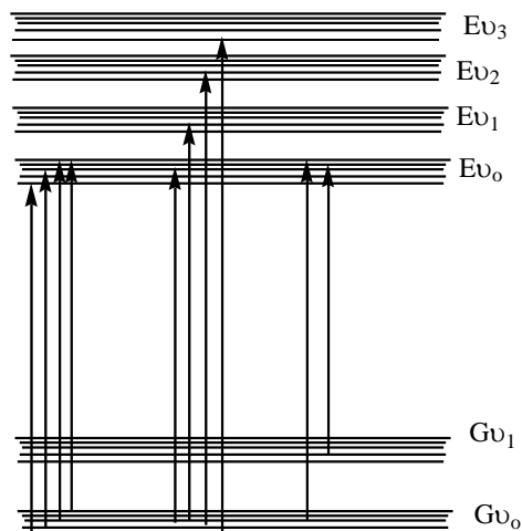
Figure 4 : Energy level diagram showing excitation between different vibrational and rotational levels of two electronic states
