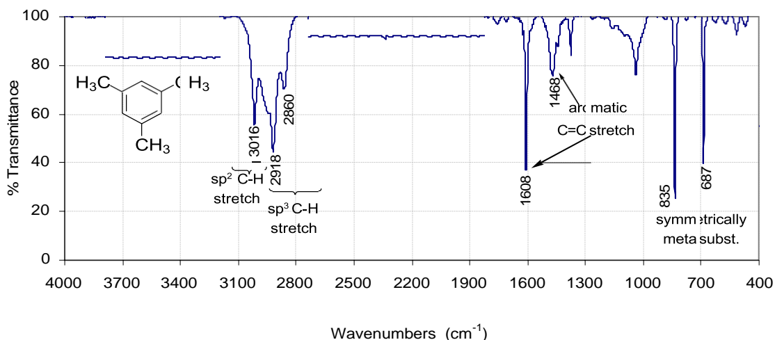
Figure 19 : The infrared spectrum of mesitylene (neat liquid)
