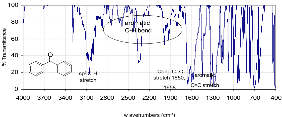
Figure 32 : The infrared spectrum of benzophenone (nujol mull)
