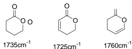
Figure 34 : Effect of conjugation in cyclic esters
